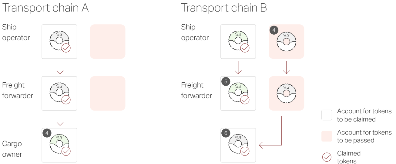
Figure 9: Resolving skipping.
