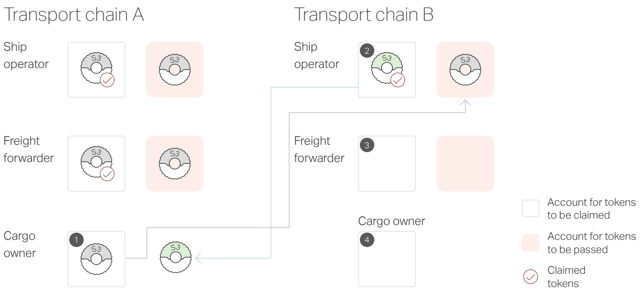
Figure 8: Skipping illustrated.
