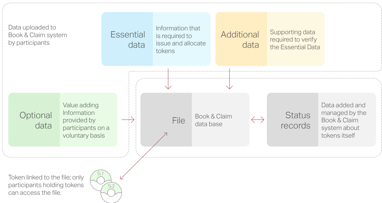
Figure 2: Token data..
