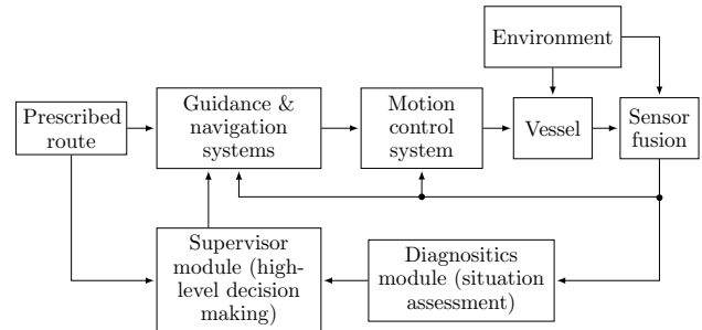
Fig. 1. Block diagram of situation awareness and navigation. Sensor information is also directly passed to the guidance and navigation systems for facilitating feedback control algorithms.
