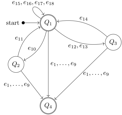
Fig. 6. State transition diagram of the decision-making automaton.
