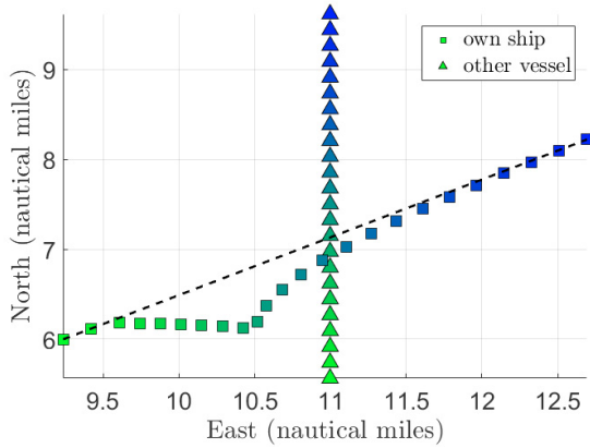
Fig. 8. Simulated courses of own ship and other vessel. The marker colours denote the evolution in time. Green colour corresponds to initial times, while blue to final times. It can be seen that the 15^\circ starboard turn of the own ship allowed the other vessel to pass from the intersection point earlier than the own ship.
